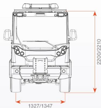
Multicar M31 with body
